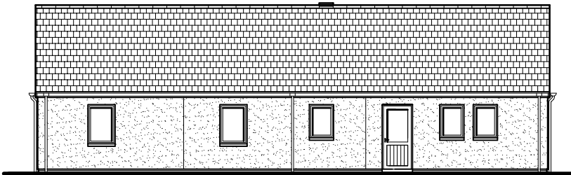
REAR ELEVATION
